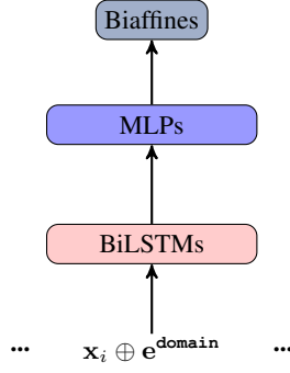
Figure 3: The framework of the DOEMB approach, where \text{domain} = \text{"src"} for source-domain sentences and \text{"tgt"} for target-domain ones.
