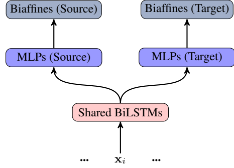
Figure 4: The framework of MTL.
